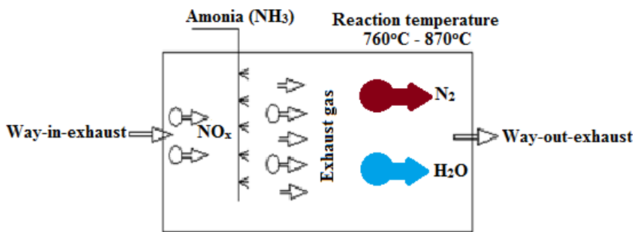
Fig.3: Principle diagram of SNCR
