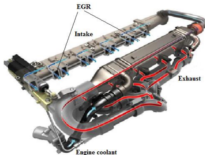
Fig.1: Principle diagram of exhaust gas recovery system
