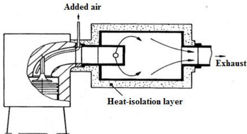
Fig.2: Principle diagram of waste heat treatment system
